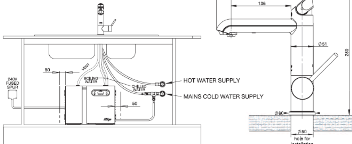
HydroTap All-In-One Commercial Non-Vented Mixer Tap
